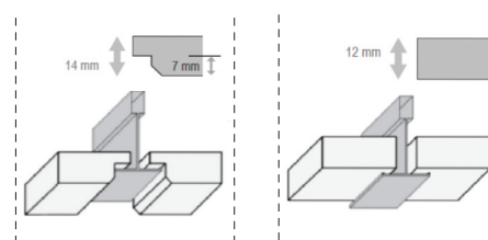
Canto Tegular
